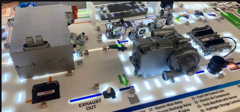
BOSCH FUEL CELL VEHICLE LAYOUT WITH COMPONENT REPLICAS
